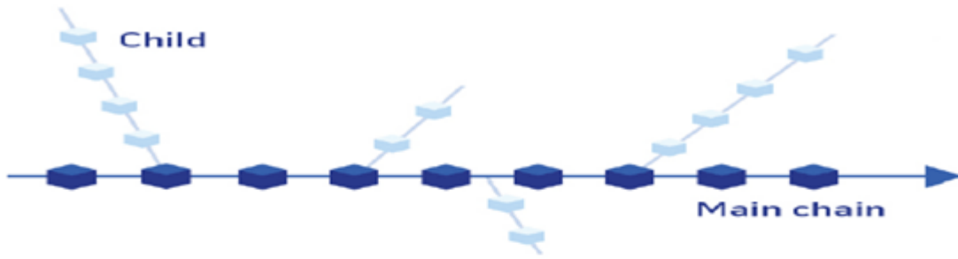
Figure 5: Multi-chain structure
