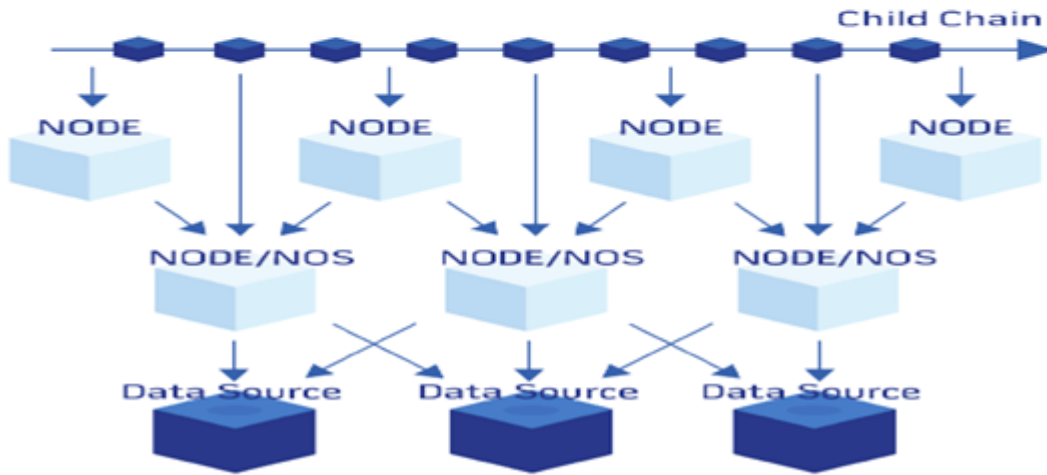
Figure 5: Multi-chain structure
